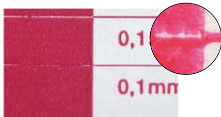
Anilox roll 100 L/cm
