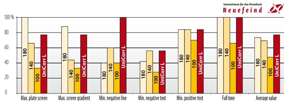
Anilox roll 180 L/cm
